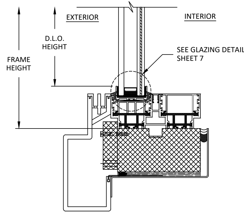
C 8 VERTICAL SECTION SILL WITH GUTTER OPTIONAL
